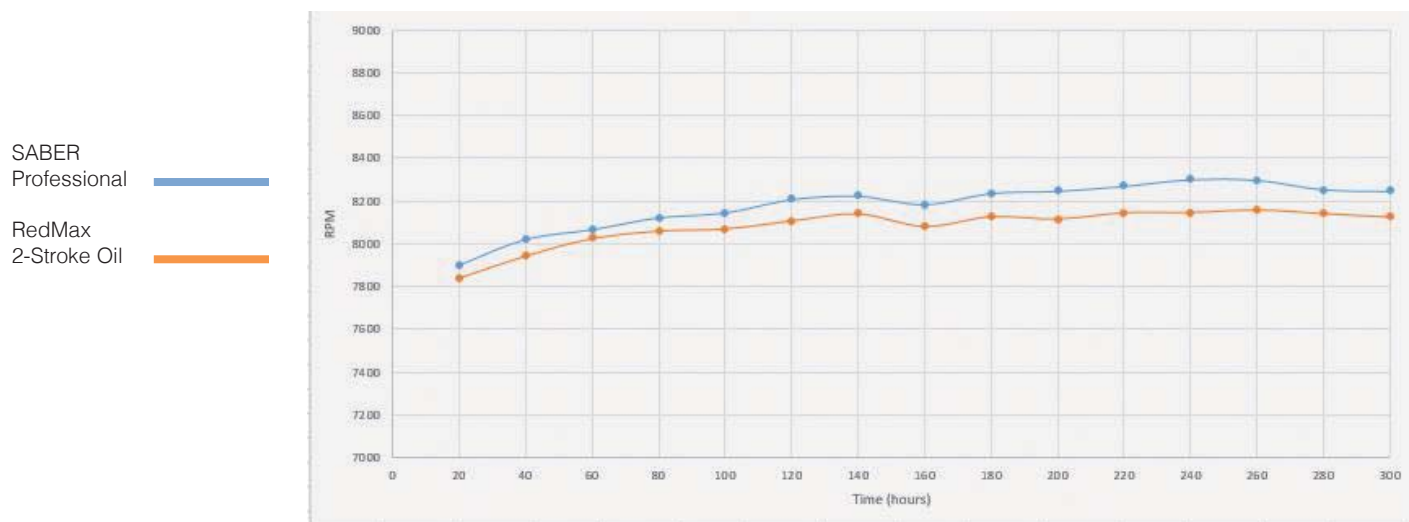
AVERAGE RPM @ WIDE-OPEN THROTTLE
